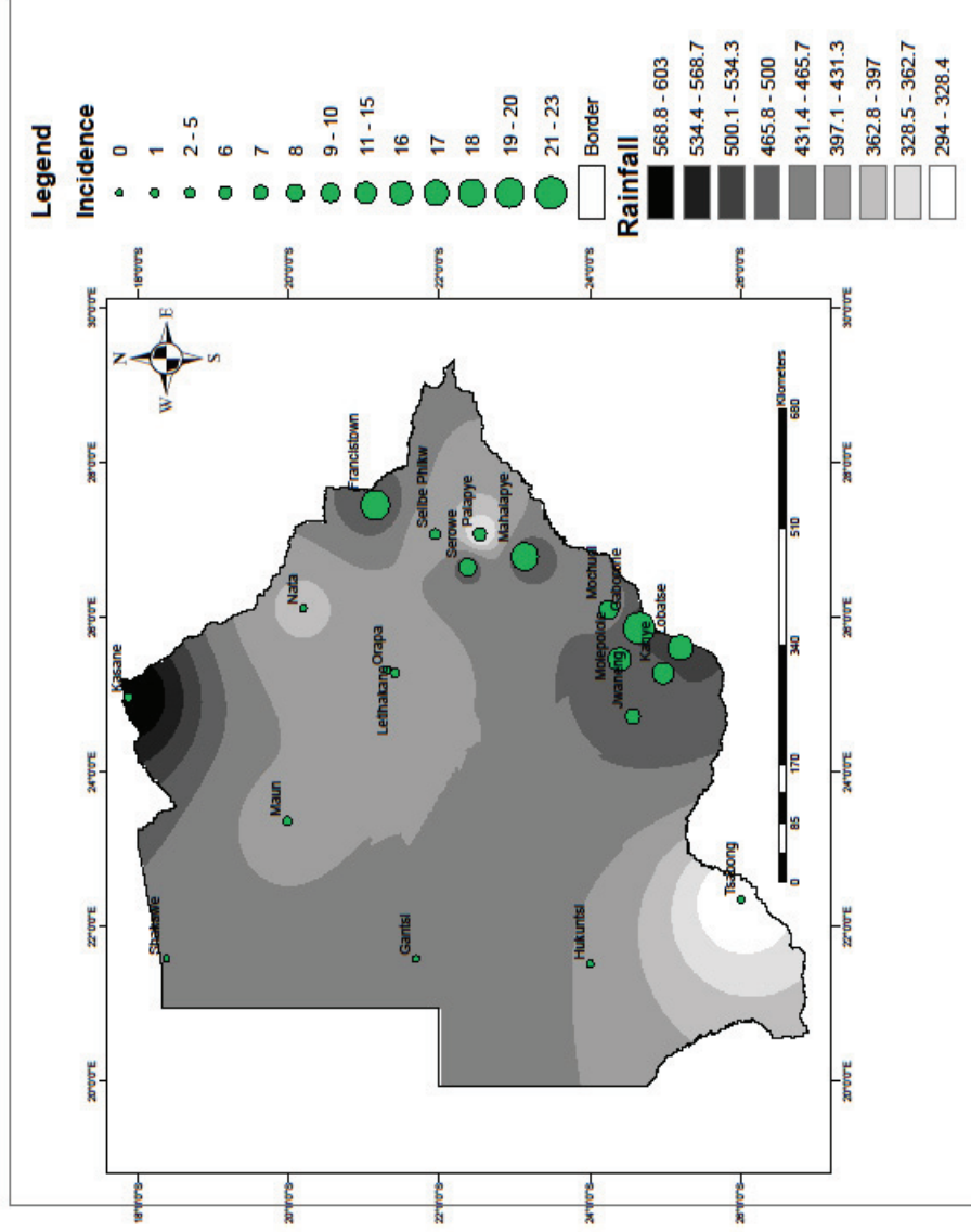
Figure 5. Spatial relationship between heartwater incidence and rainfall amount
